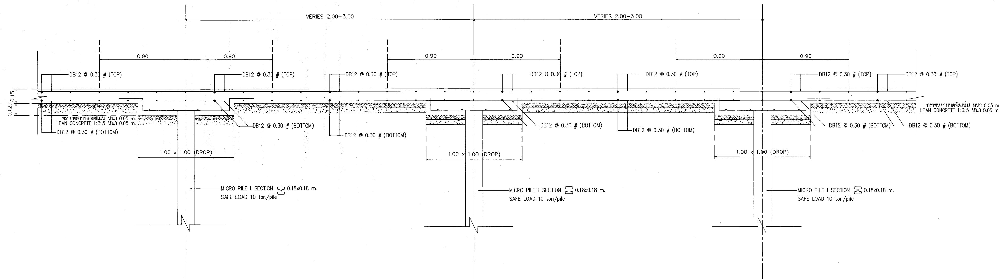
DETAILED SHORT SPAN OF FS. 1:20
